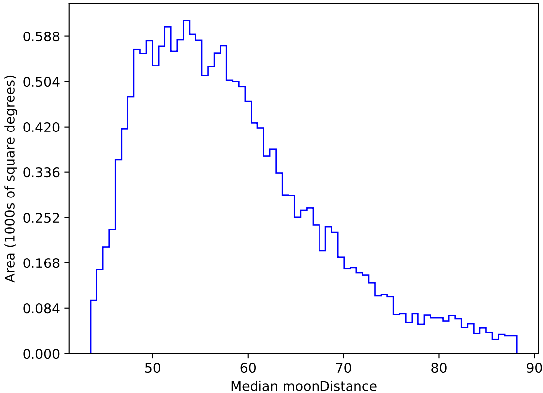
weather_cloudso4v3.4_10yrs WFD y band: Median moonDistance
