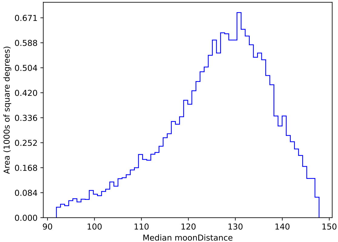
weather_cloudso4v3.4_10yrs WFD u band: Median moonDistance
