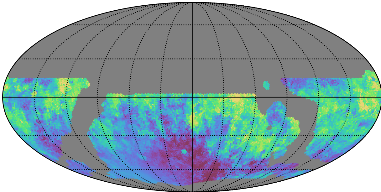
weather_cloudso4v3.4_10yrs WFD i band: Median moonDistance
