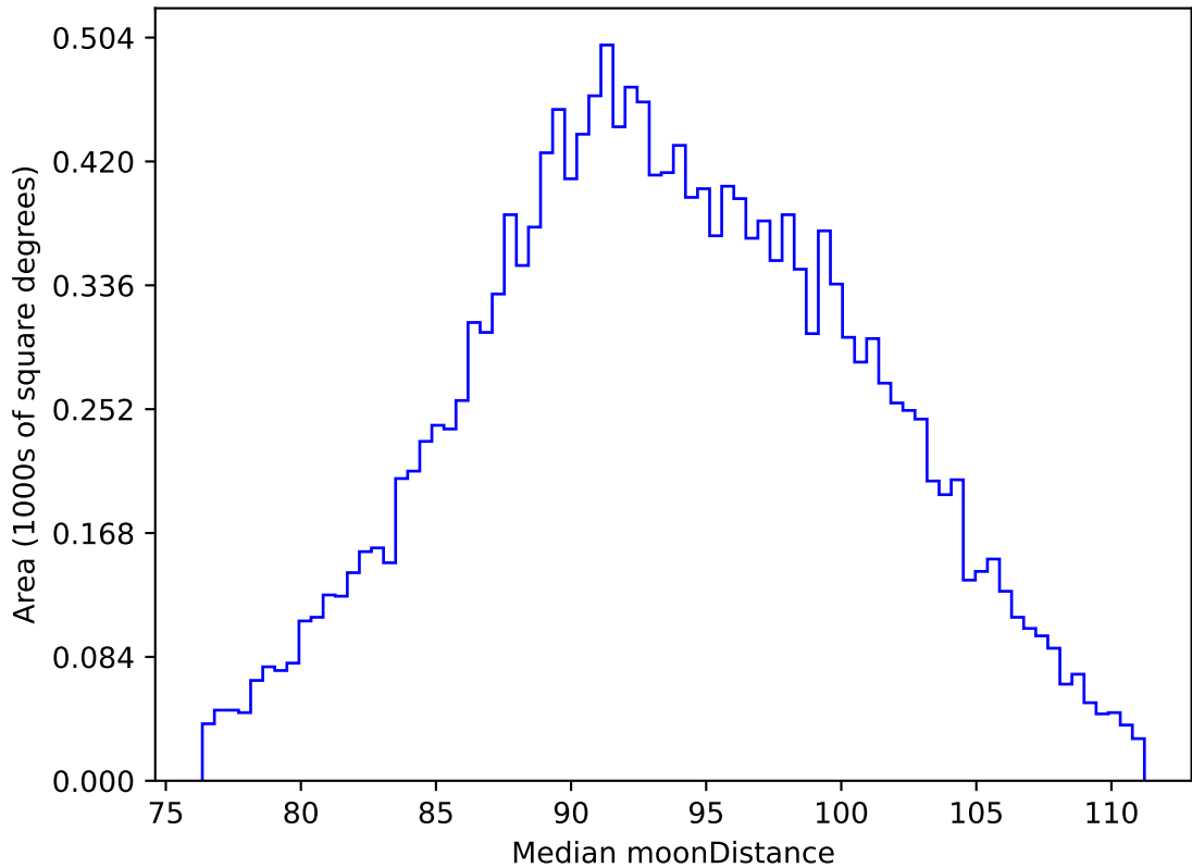
weather_cloudso4v3.4_10yrs WFD i band: Median moonDistance
