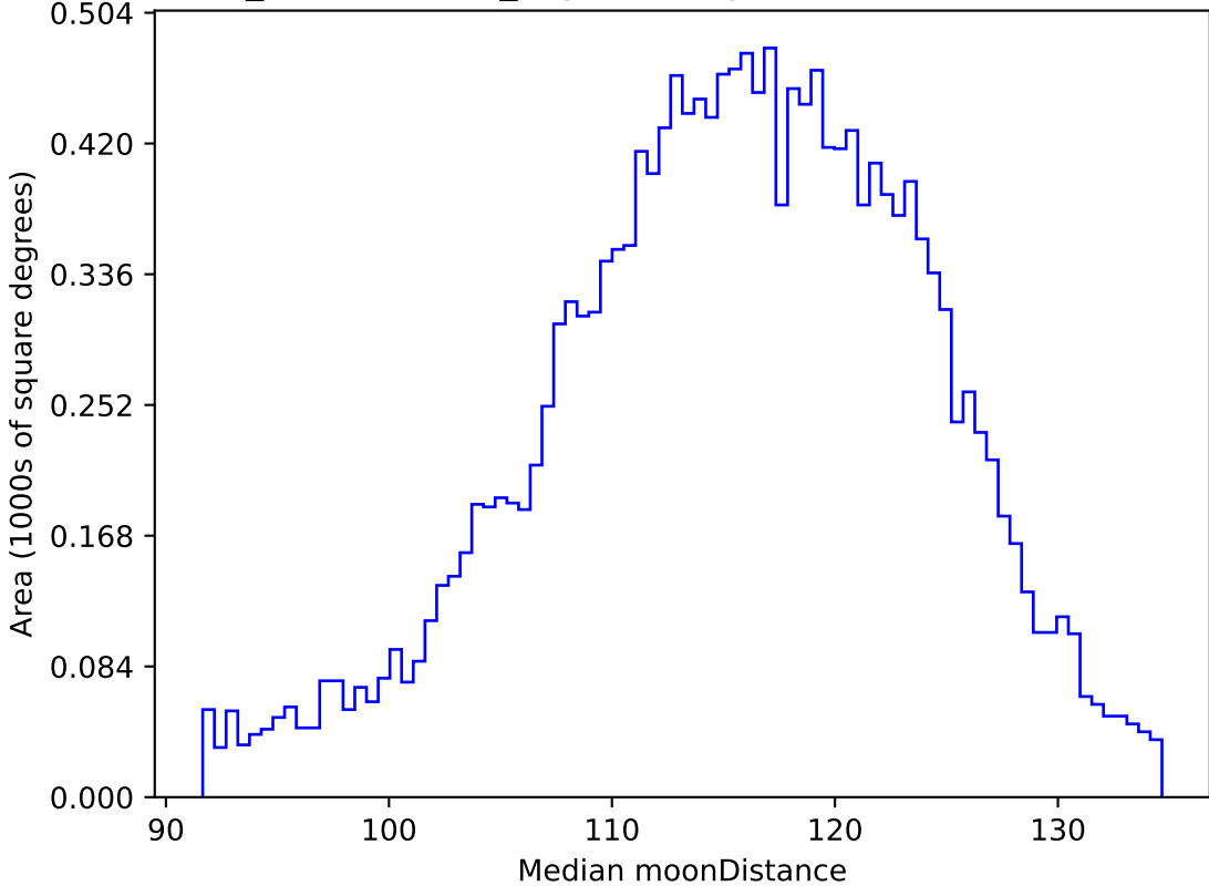
weather_cloudso4v3.4_10yrs WFD g band: Median moonDistance
