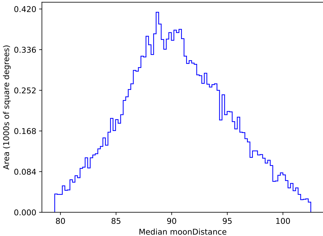
weather_cloudso4v3.4_10yrs WFD all bands: Median moonDistance
