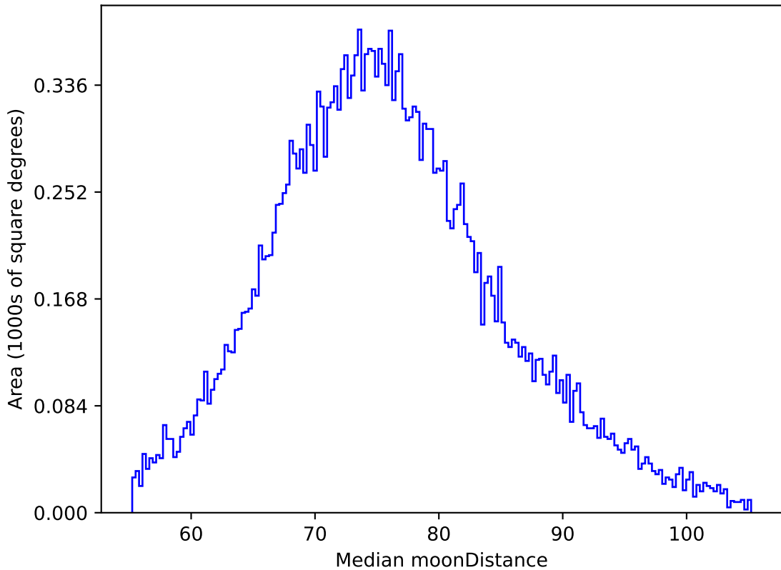
weather_cloudso4v3.4_10yrs All sky z band: Median moonDistance
