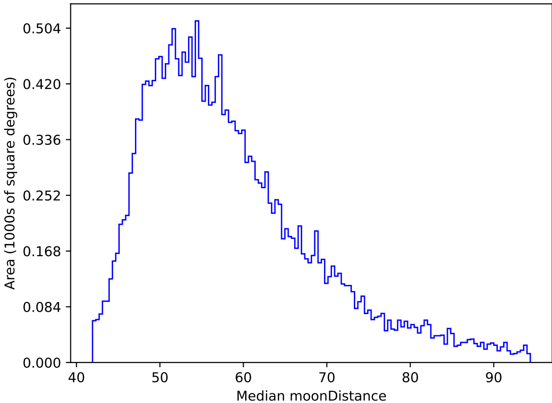
weather_cloudso4v3.4_10yrs All sky y band: Median moonDistance
