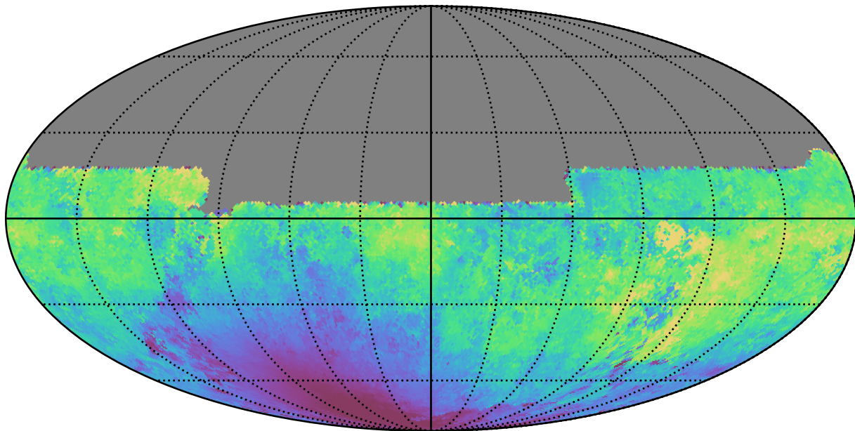
weather_cloudso4v3.4_10yrs All sky u band: Median moonDistance
