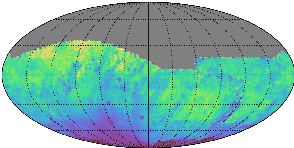
weather_cloudso4v3.4_10yrs All sky r band: Median moonDistance
