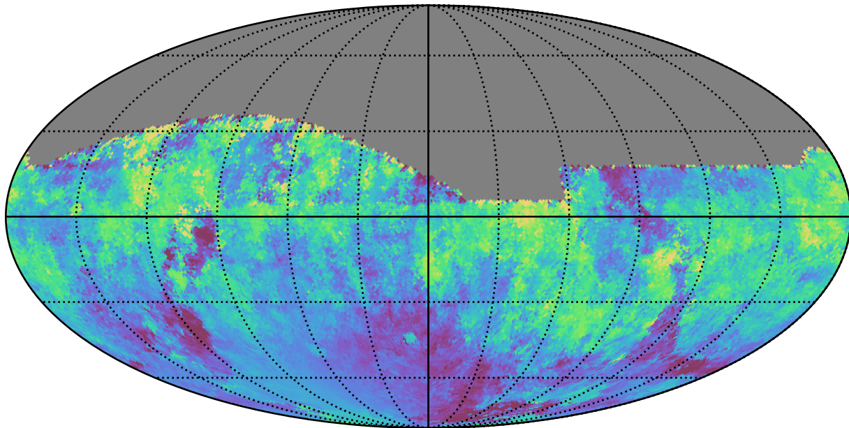
weather_cloudso4v3.4_10yrs All sky i band: Median moonDistance
