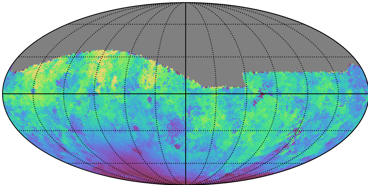
weather_cloudso4v3.4_10yrs All sky g band: Median moonDistance
