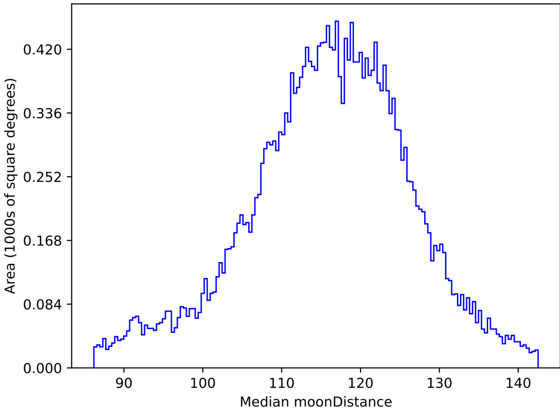
weather_cloudso4v3.4_10yrs All sky g band: Median moonDistance
