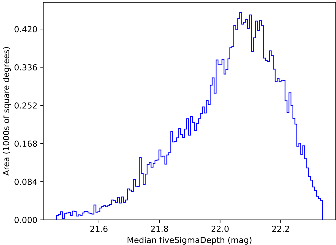
weather_cloudso4v3.4_10yrs Yr 1 y band: Median fiveSigmaDepth
