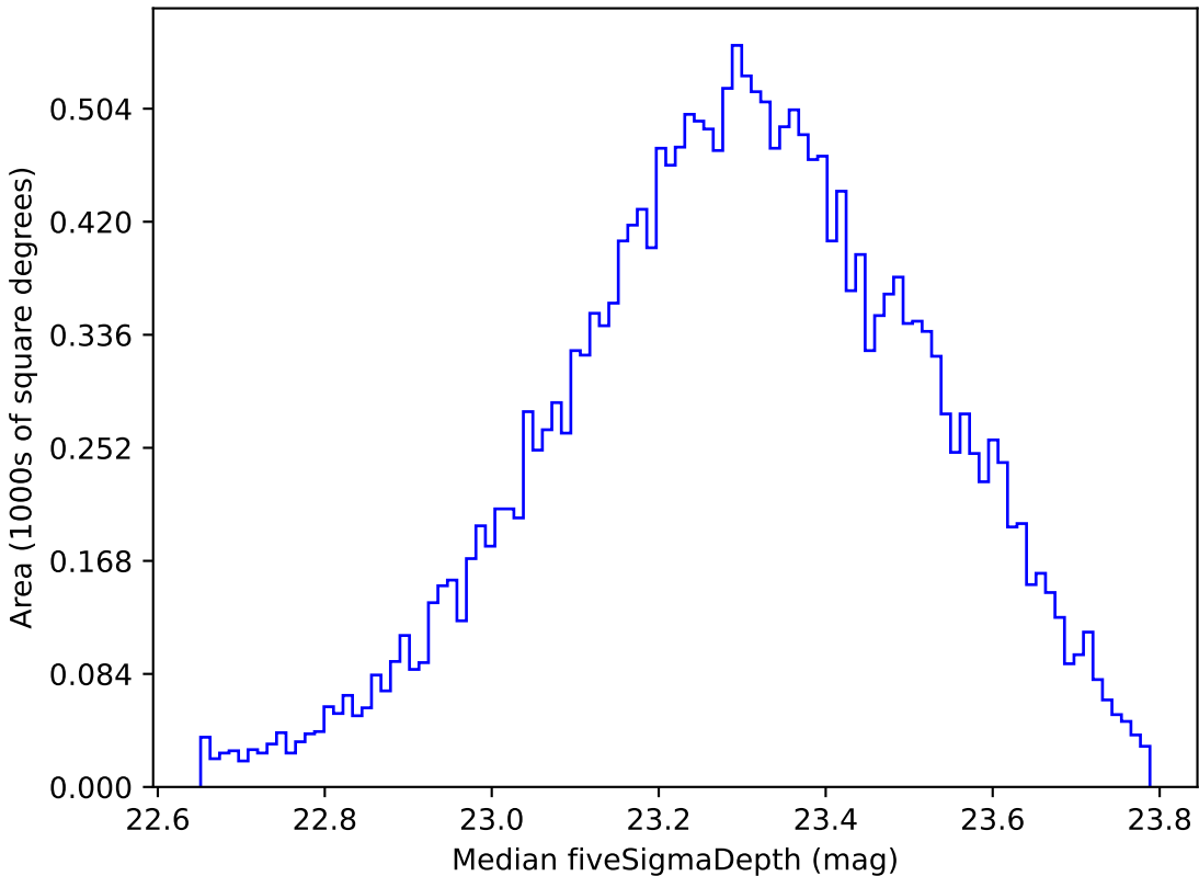
weather_cloudso4v3.4_10yrs Yr 1 u band: Median fiveSigmaDepth
