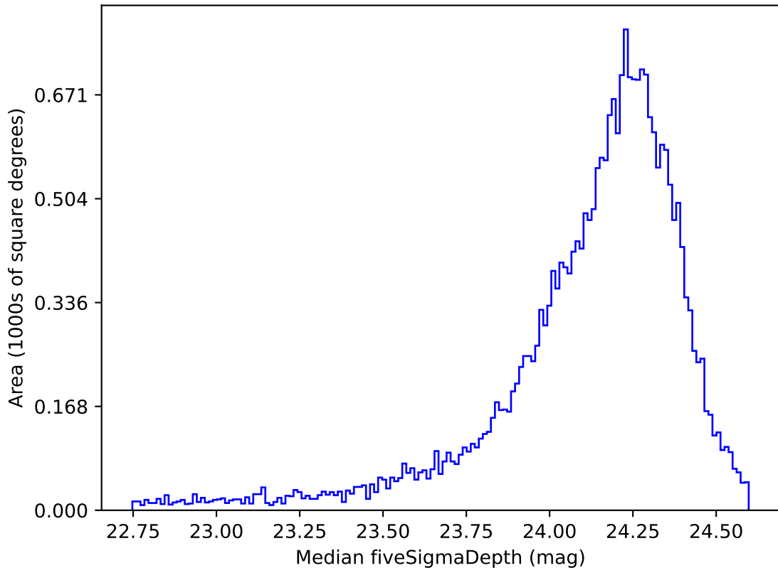
weather_cloudso4v3.4_10yrs Yr 1 r band: Median fiveSigmaDepth
