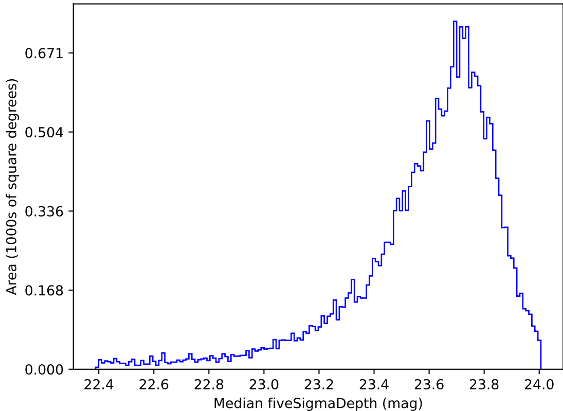
weather_cloudso4v3.4_10yrs Yr 1 i band: Median fiveSigmaDepth
