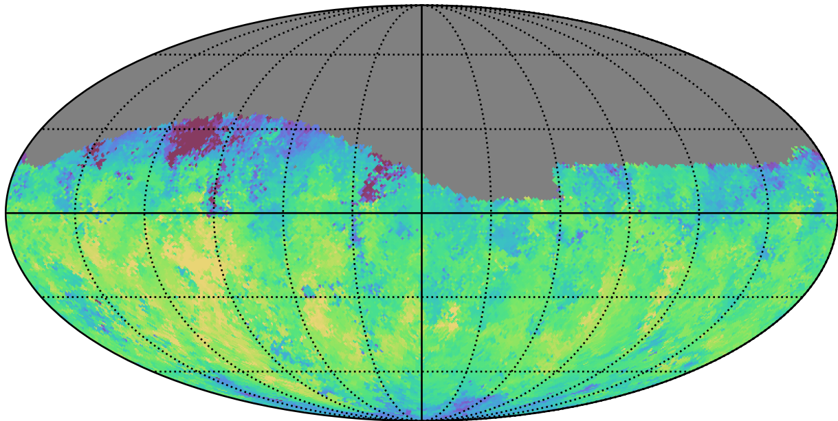
weather_cloudso4v3.4_10yrs Yr 1 g band: Median fiveSigmaDepth
