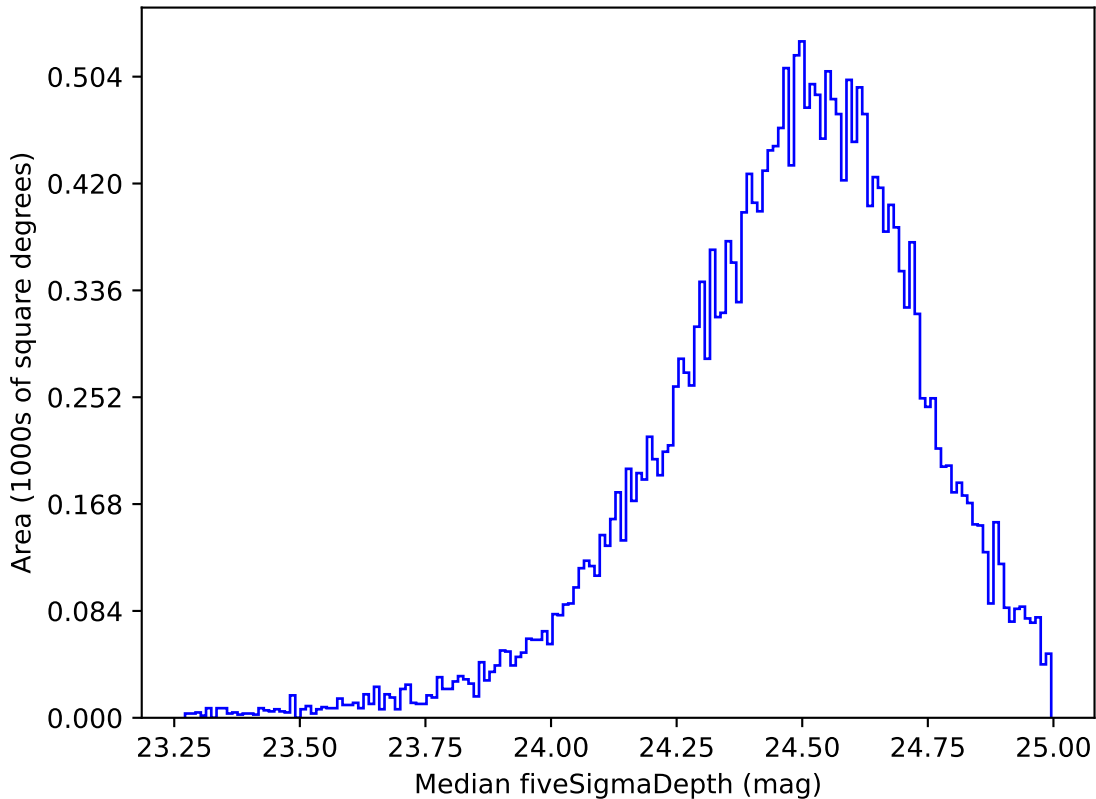
weather_cloudso4v3.4_10yrs Yr 1 g band: Median fiveSigmaDepth
