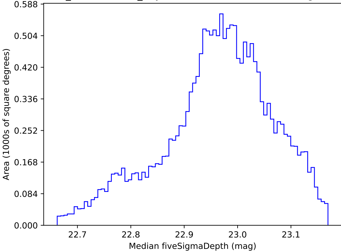
weather_cloudso4v3.4_10yrs WFD z band: Median fiveSigmaDepth
