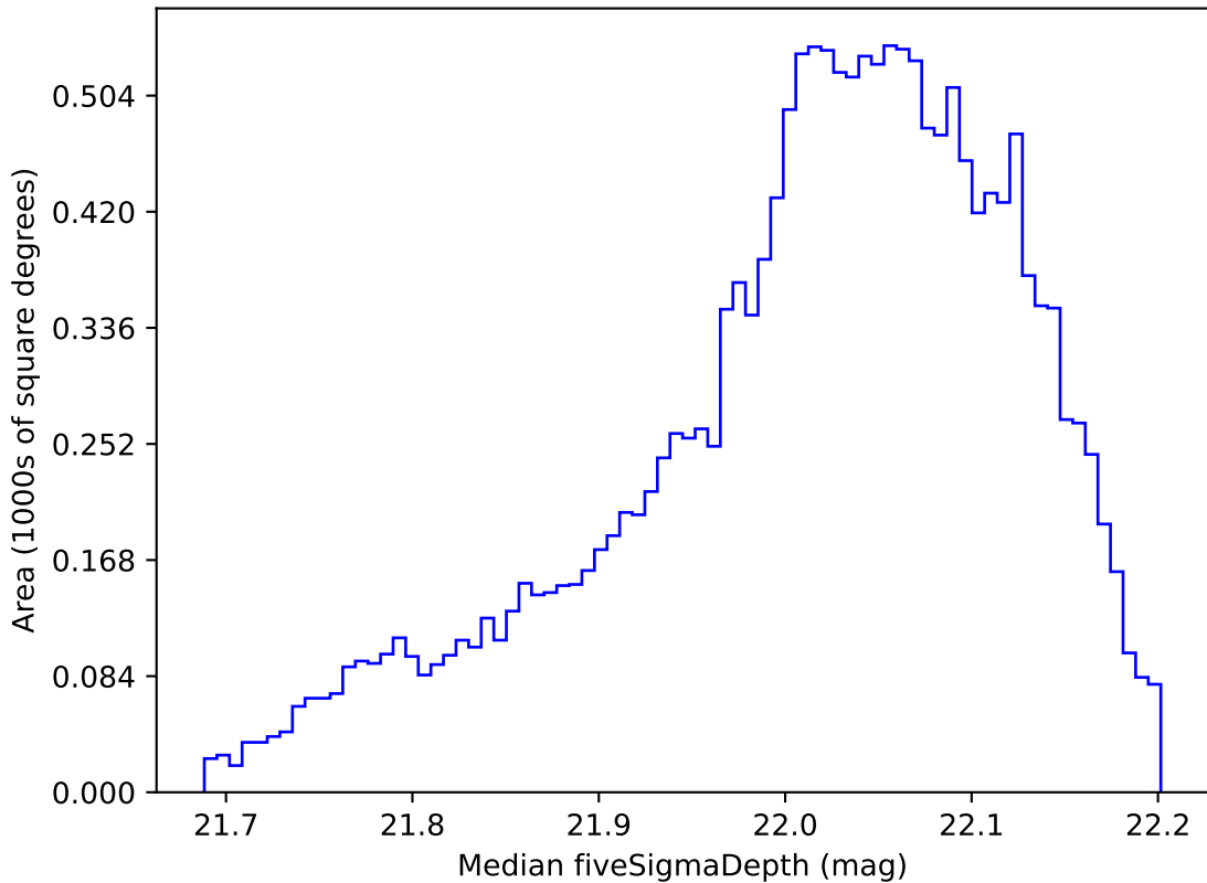
weather_cloudso4v3.4_10yrs WFD y band: Median fiveSigmaDepth
