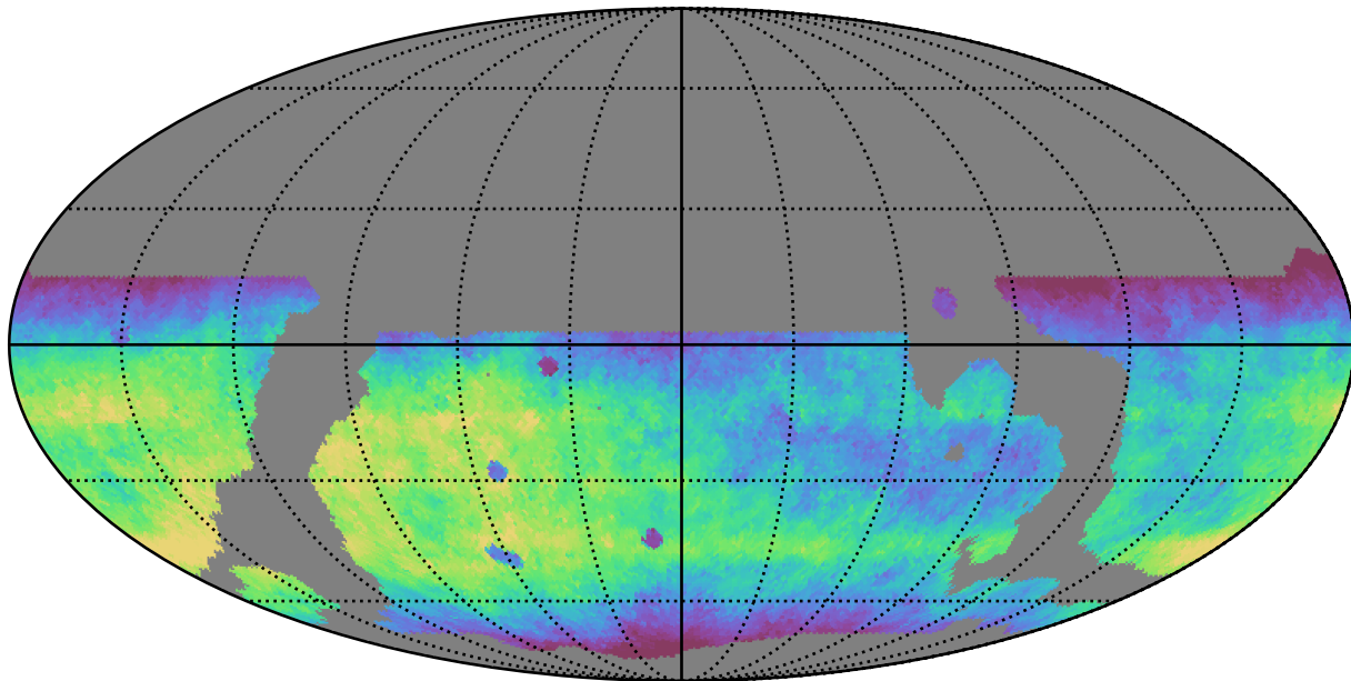
weather_cloudso4v3.4_10yrs WFD r band: Median fiveSigmaDepth
