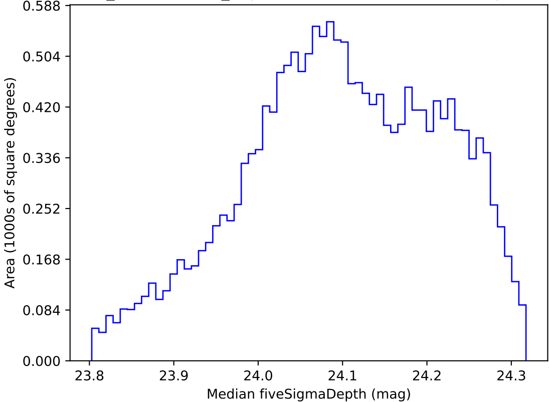
weather_cloudso4v3.4_10yrs WFD r band: Median fiveSigmaDepth
