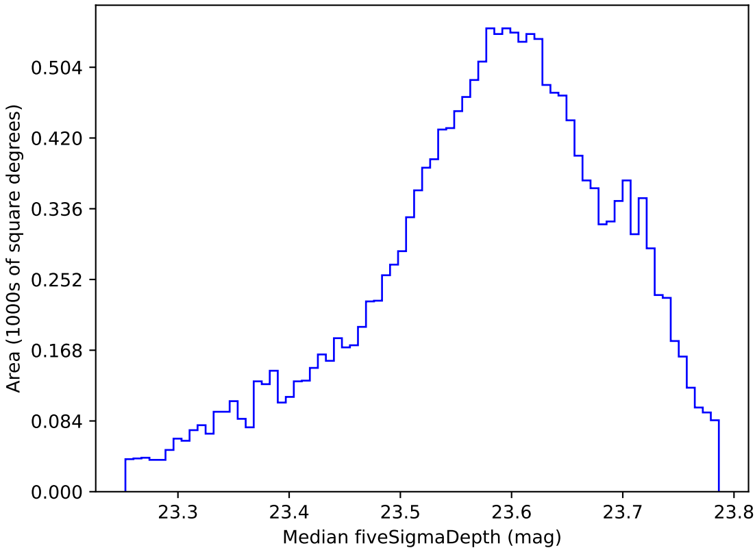
weather_cloudso4v3.4_10yrs WFD i band: Median fiveSigmaDepth
