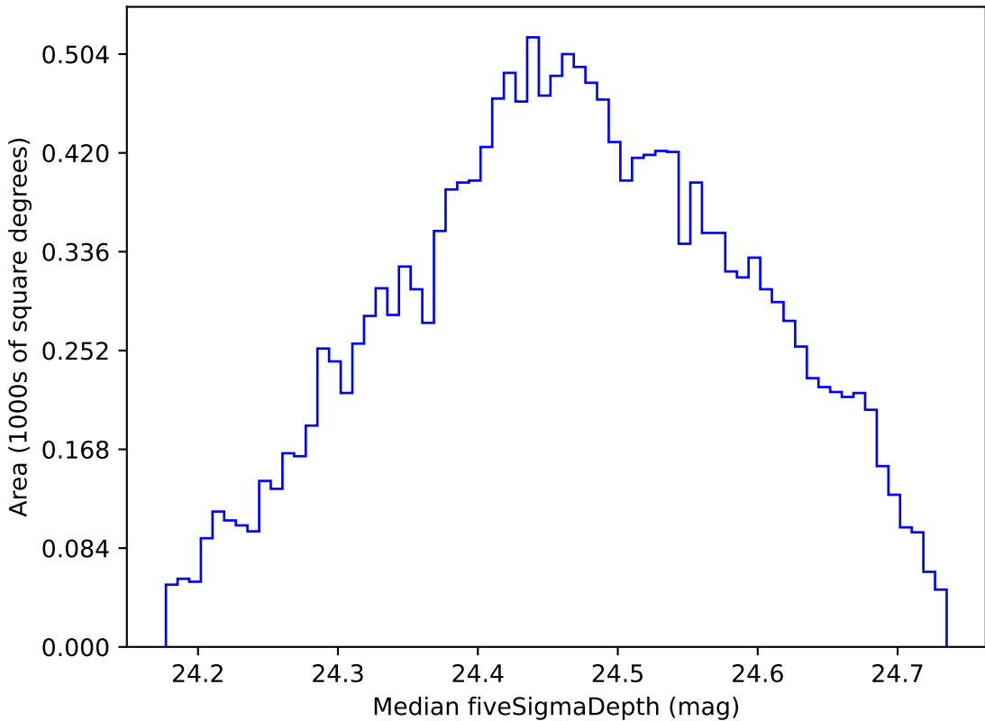
weather_cloudso4v3.4_10yrs WFD g band: Median fiveSigmaDepth
