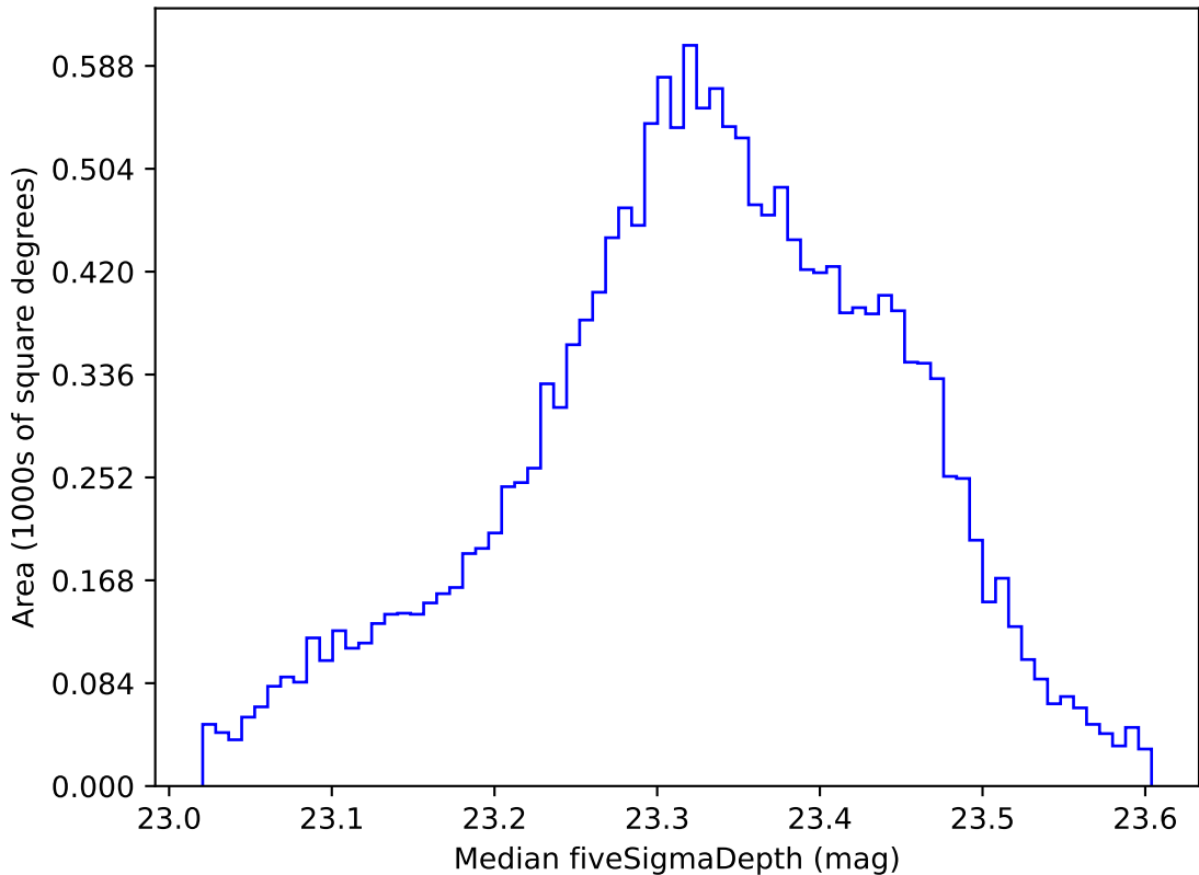
weather_cloudso4v3.4_10yrs WFD all bands: Median fiveSigmaDepth
