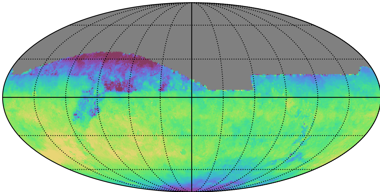
weather_cloudso4v3.4_10yrs All sky z band: Median fiveSigmaDepth
