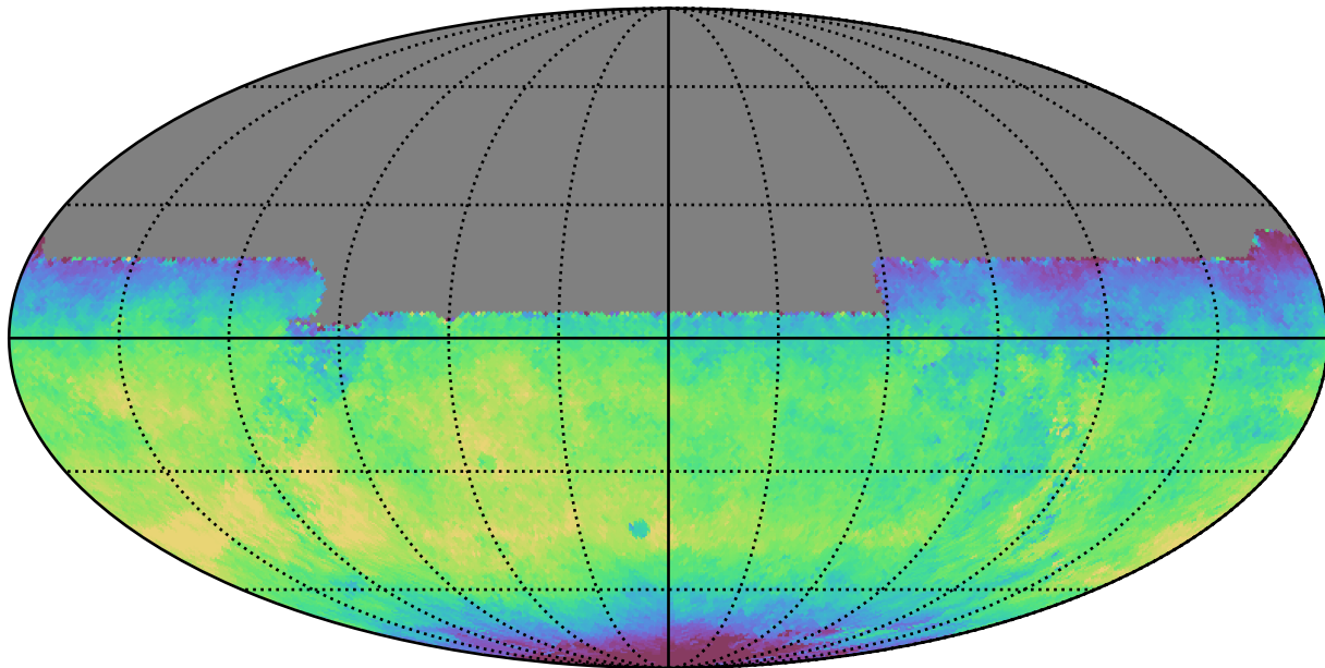
weather_cloudso4v3.4_10yrs All sky y band: Median fiveSigmaDepth
