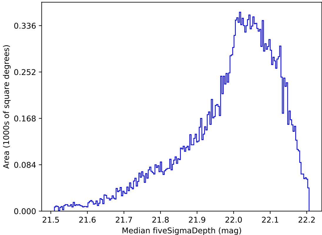
weather_cloudso4v3.4_10yrs All sky y band: Median fiveSigmaDepth
