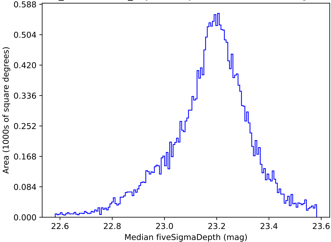
weather_cloudso4v3.4_10yrs All sky u band: Median fiveSigmaDepth
