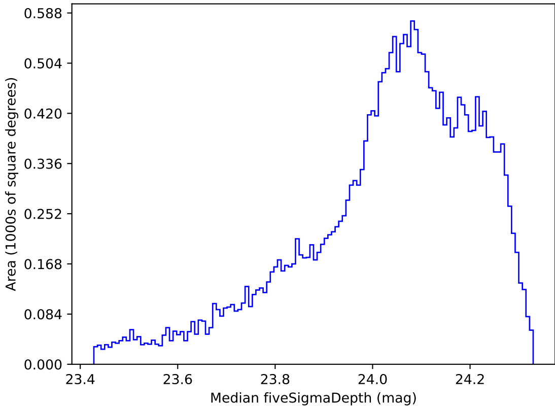
weather_cloudso4v3.4_10yrs All sky r band: Median fiveSigmaDepth
