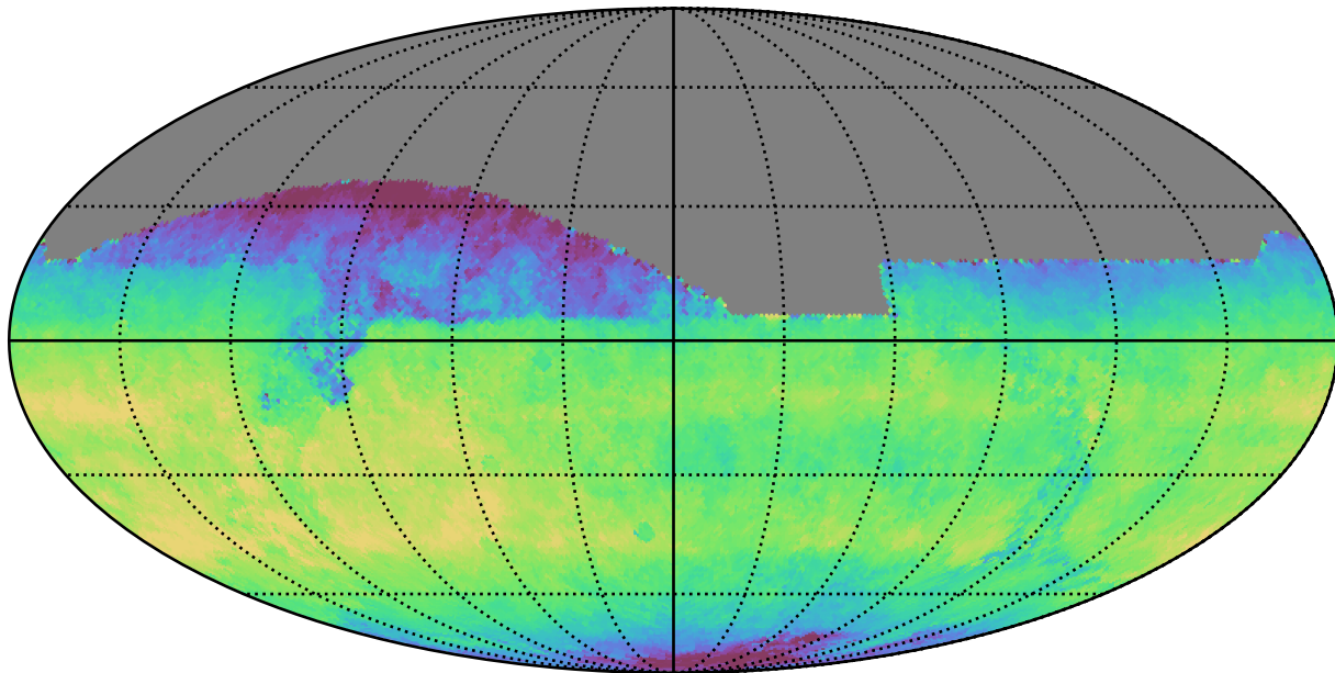
weather_cloudso4v3.4_10yrs All sky i band: Median fiveSigmaDepth
