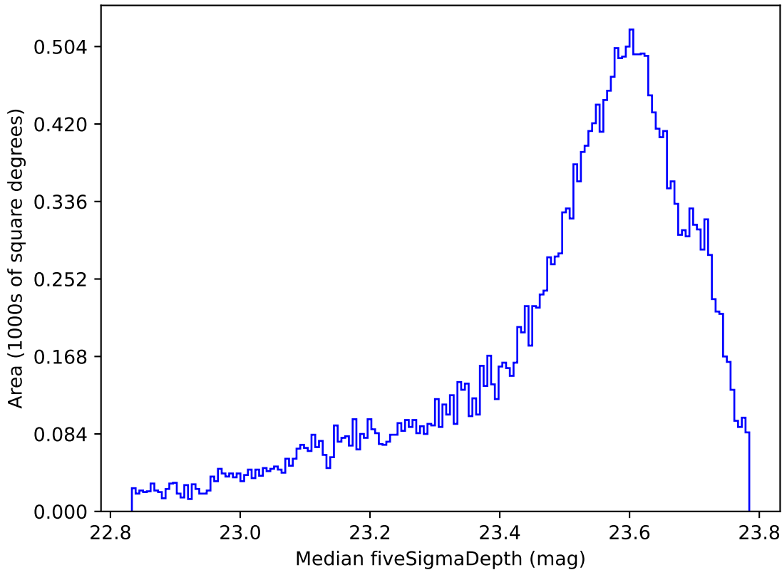
weather_cloudso4v3.4_10yrs All sky i band: Median fiveSigmaDepth
