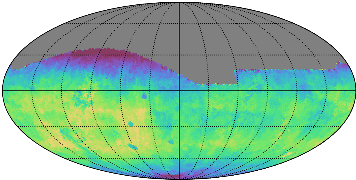
weather_cloudso4v3.4_10yrs All sky g band: Median fiveSigmaDepth
