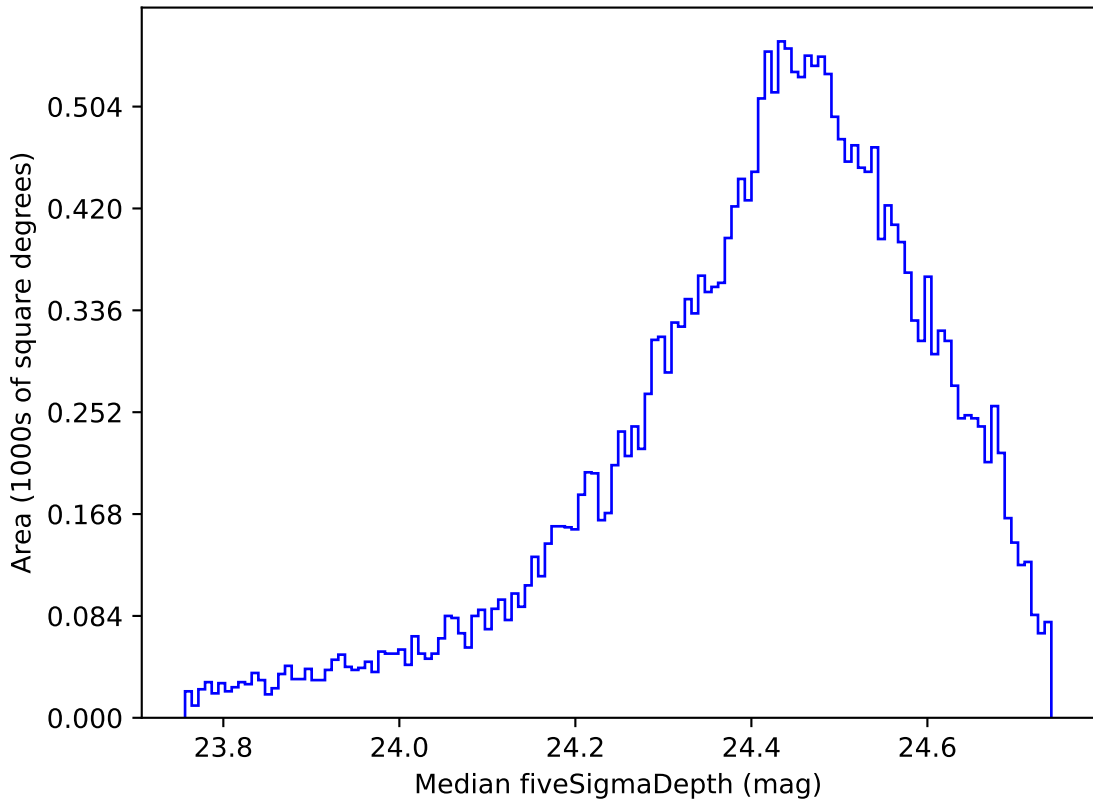
weather_cloudso4v3.4_10yrs All sky g band: Median fiveSigmaDepth
