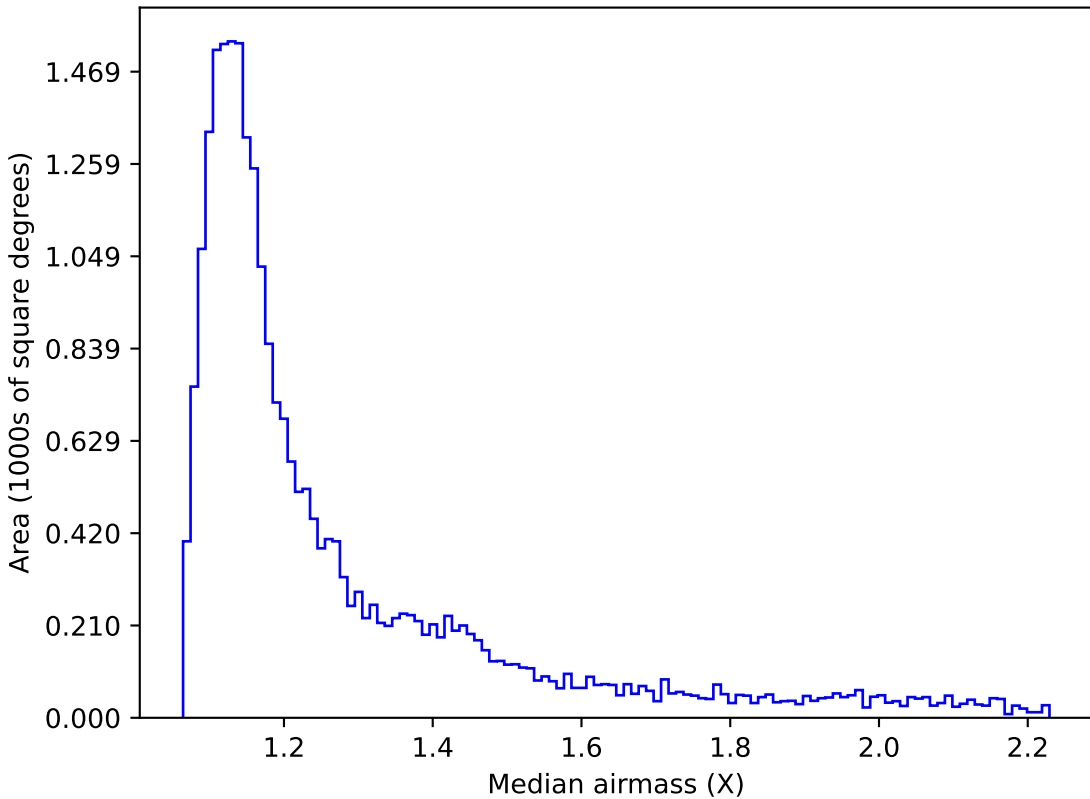
weather_cloudso4v3.4_10yrs Yr 1 z band: Median airmass
