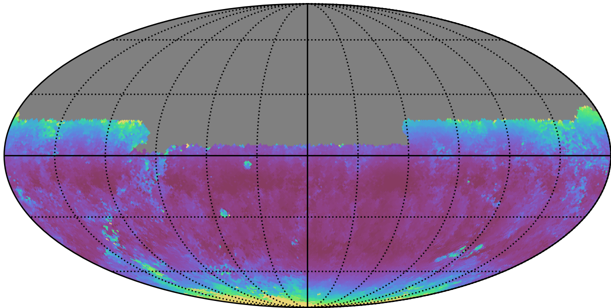
weather_cloudso4v3.4_10yrs Yr 1 y band: Median airmass
