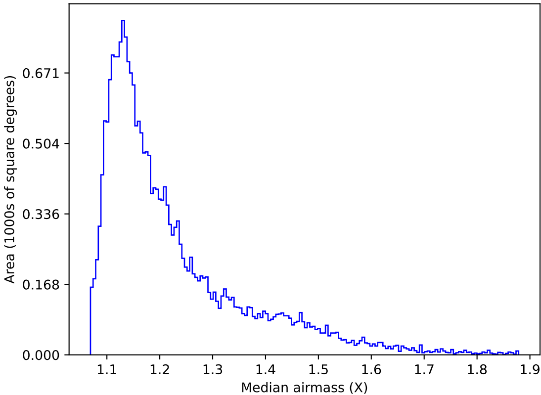
weather_cloudso4v3.4_10yrs Yr 1 y band: Median airmass
