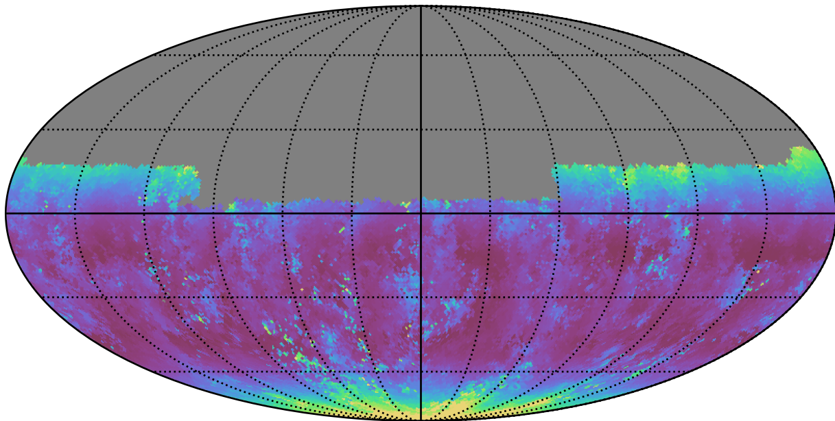
weather_cloudso4v3.4_10yrs Yr 1 u band: Median airmass
