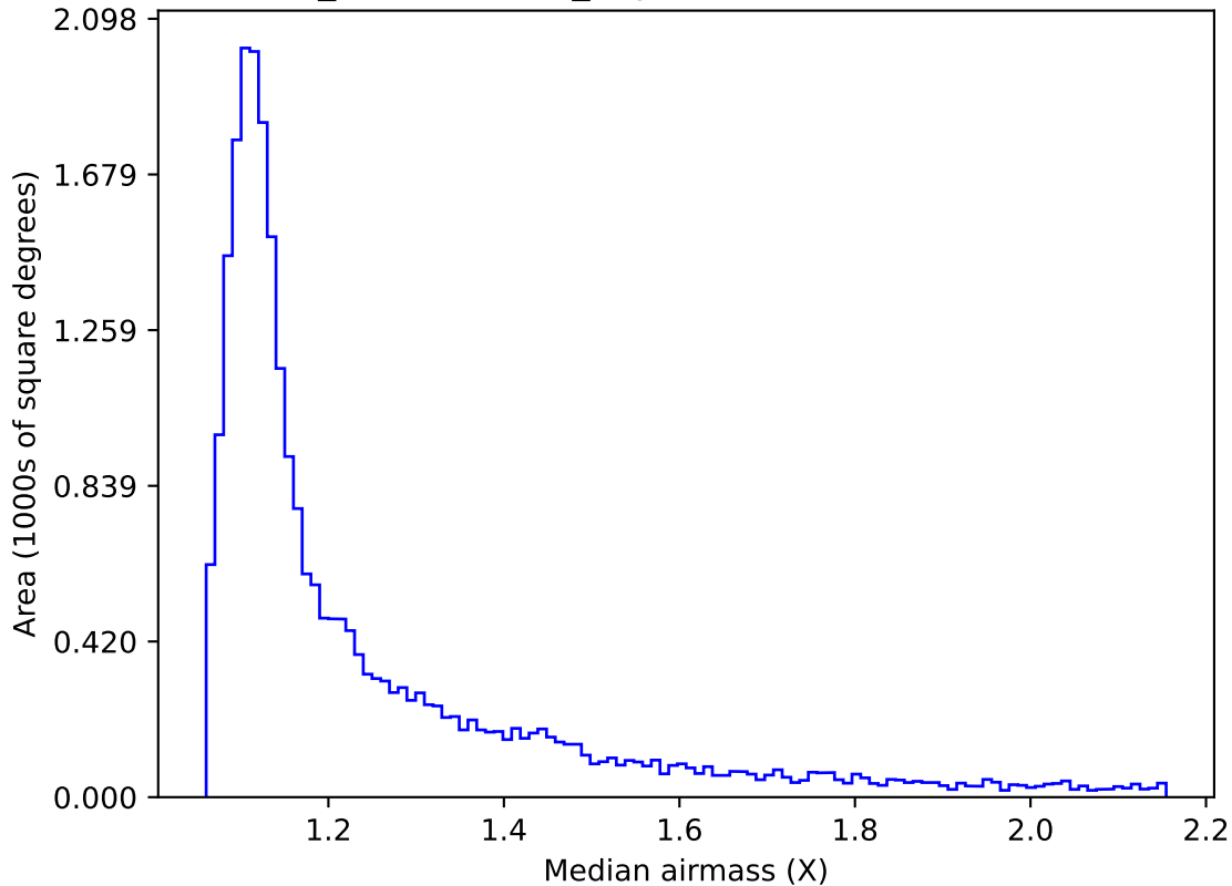
weather_cloudso4v3.4_10yrs Yr 1 r band: Median airmass
