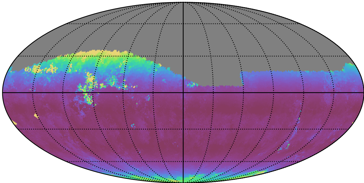
weather_cloudso4v3.4_10yrs Yr 1 i band: Median airmass
