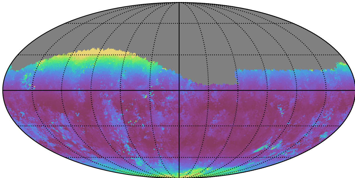
weather_cloudso4v3.4_10yrs Yr 1 g band: Median airmass
