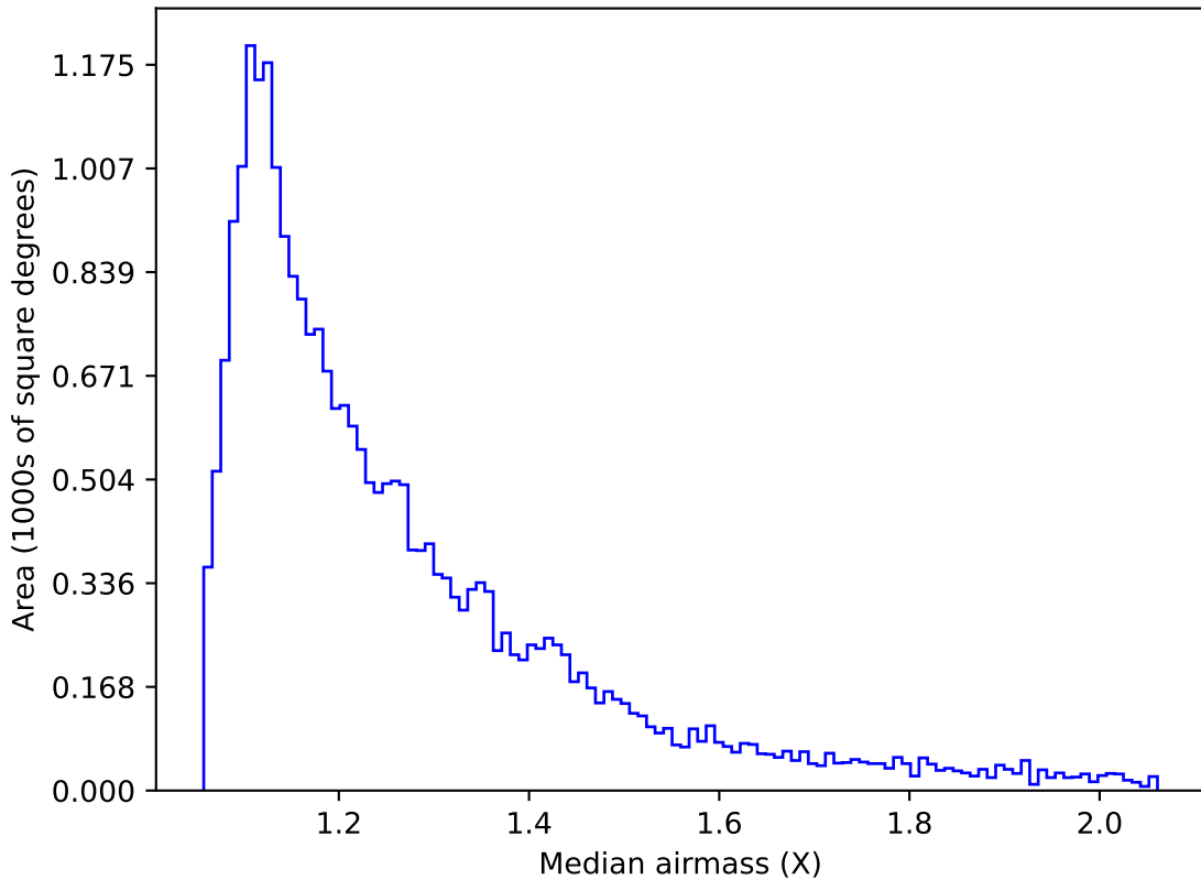
weather_cloudso4v3.4_10yrs Yr 1 g band: Median airmass
