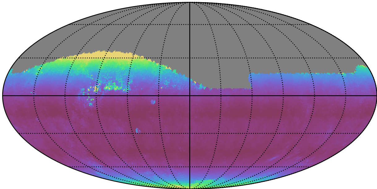
weather_cloudso4v3.4_10yrs Yr 1 all bands: Median airmass
