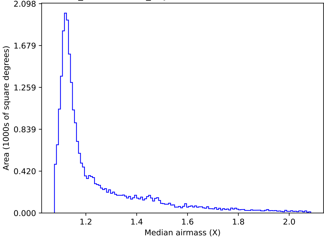
weather_cloudso4v3.4_10yrs Yr 1 all bands: Median airmass
