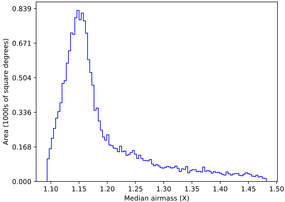
weather_cloudso4v3.4_10yrs WFD z band: Median airmass
