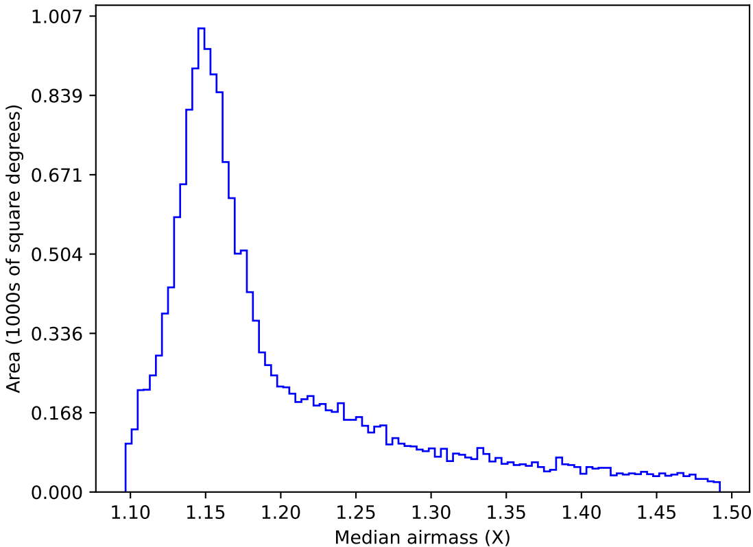
weather_cloudso4v3.4_10yrs WFD y band: Median airmass
