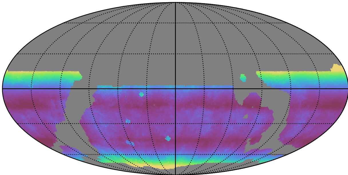
weather_cloudso4v3.4_10yrs WFD r band: Median airmass
