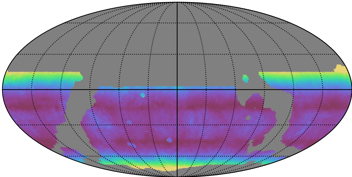
weather_cloudso4v3.4_10yrs WFD i band: Median airmass
