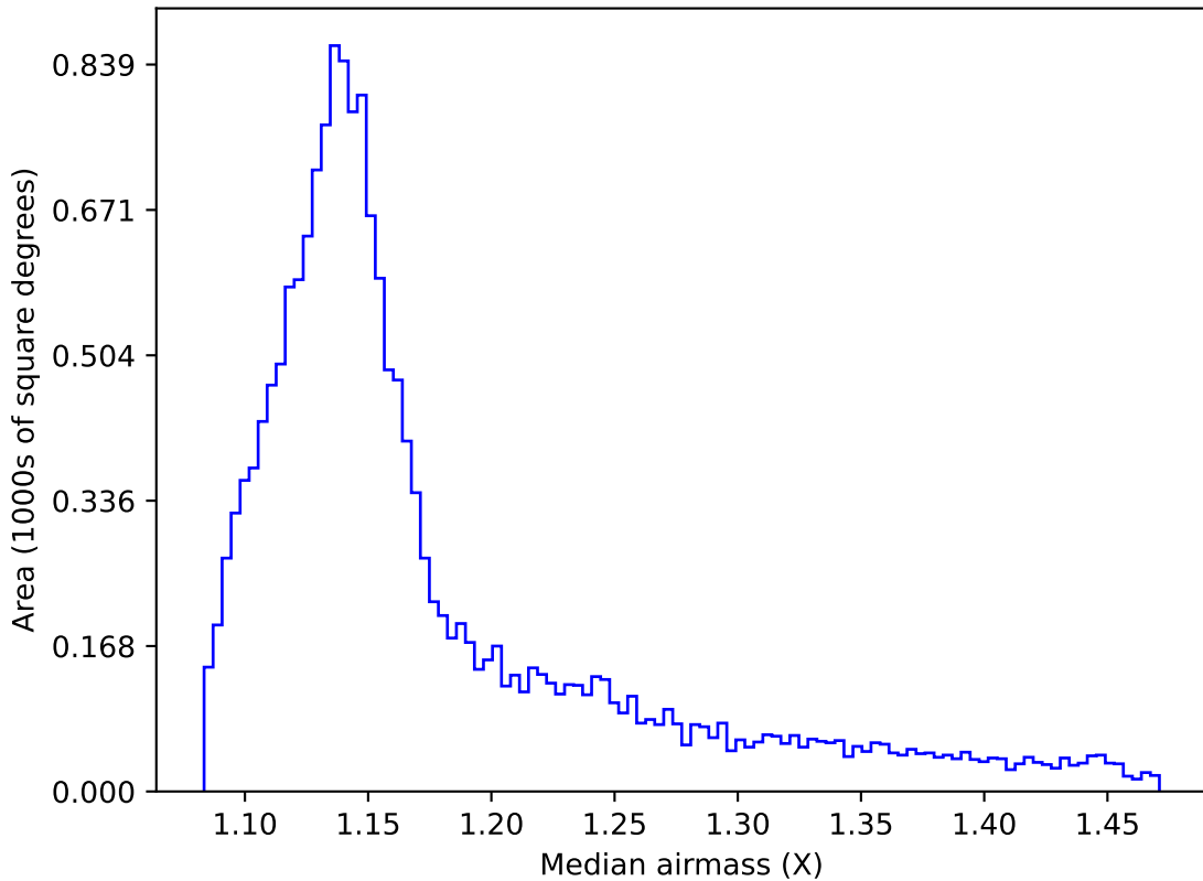
weather_cloudso4v3.4_10yrs WFD i band: Median airmass
